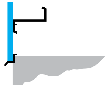
Base Girt / Base Trim
