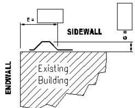
TIE-IN CORNER
