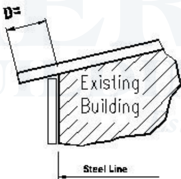
EAVE OVERHANG
